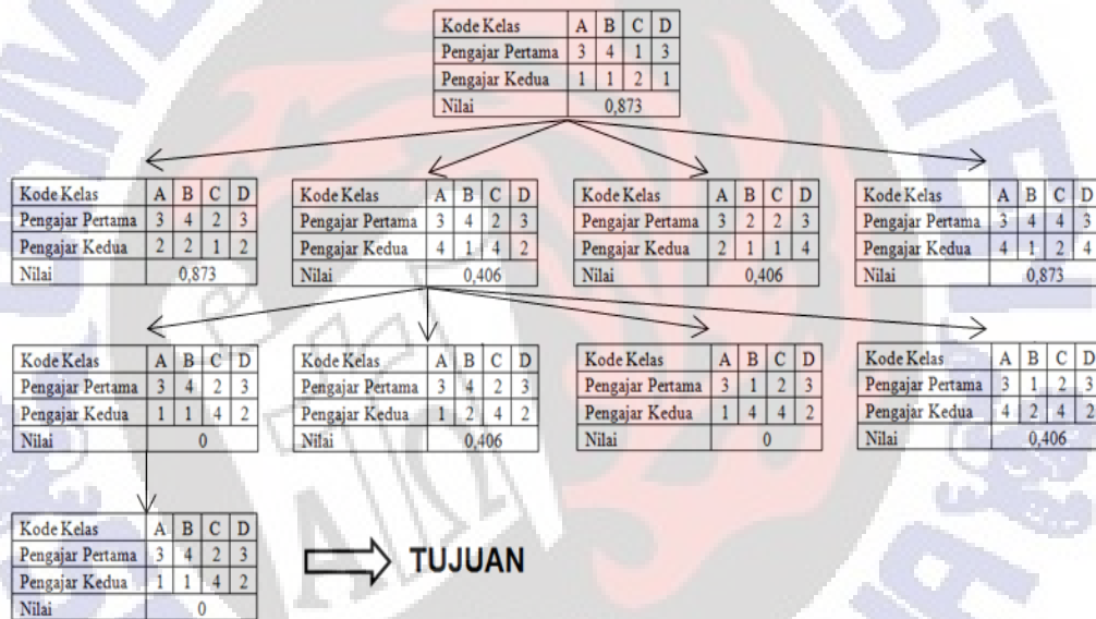
Gambar 2 Ilustrasi Alur Algoritma Steepest Ascent Hill Climbing
